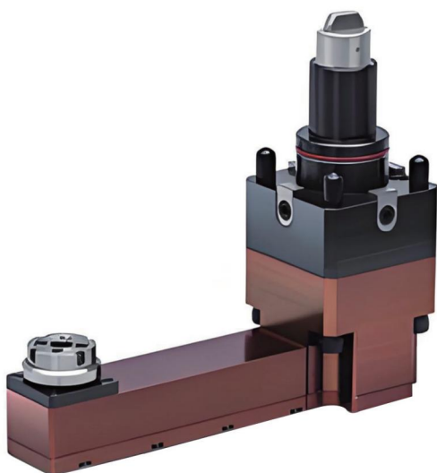
Internal slotted power tool holder
